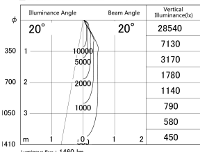
■ Direct Horizontal Illuminance DD140-1520WW9040D
