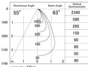
■ Direct Horizontal Illuminance DD140-0850WB9027D
