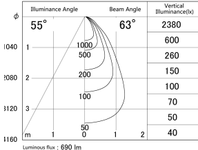
■ Direct Horizontal Illuminance DD140-0850WB9030D
