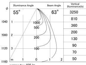
■ Direct Horizontal Illuminance DD140-1050WB9035D
