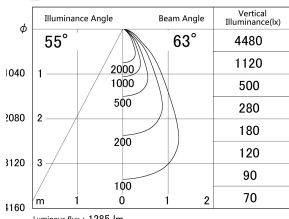
■ Direct Horizontal Illuminance DD140-1550WB9035D
