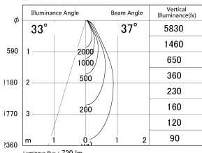
■ Direct Horizontal Illuminance DD140-0830WB9040D
