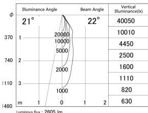
■ Direct Horizontal Illuminance DD139-2520MW9027
