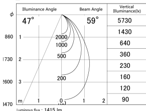
■ Direct Horizontal Illuminance DD139-1550MW9030
