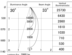
■ Direct Horizontal Illuminance DD139-3030MW9035
