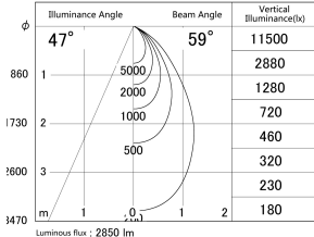
■ Direct Horizontal Illuminance DD139-3050MW9040
