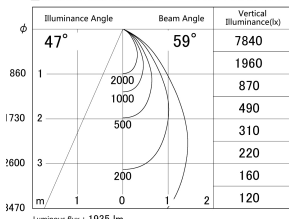
■ Direct Horizontal Illuminance DD139-2050MB9027
