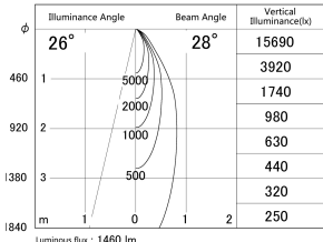
■ Direct Horizontal Illuminance DD139-1520MB9030
