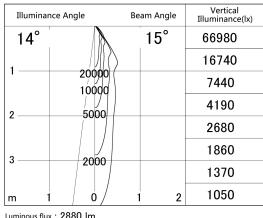
■ Direct Horizontal Illuminance DD139-3015MB9030
