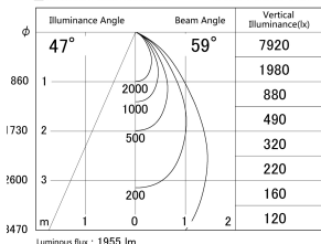
■ Direct Horizontal Illuminance DD139-2050MB9035
