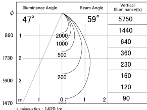
■ Direct Horizontal Illuminance DD139-1550MB9040
