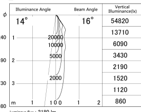
■ Direct Horizontal Illuminance DD139-2015MB9040
