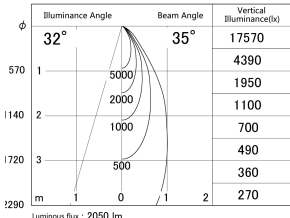
■ Direct Horizontal Illuminance DD139-2030MB9040
