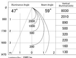
■ Direct Horizontal Illuminance DD139-2050MB9040
