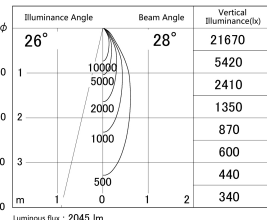
■ Direct Horizontal Illuminance DD139-2020DW9035
