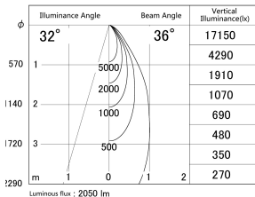
■ Direct Horizontal Illuminance DD139-2030DW9035
