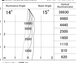
■ Direct Horizontal Illuminance DD139-1515DW9040
