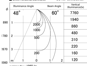
■ Direct Horizontal Illuminance DD139-2050DB9027
