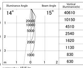
■ Direct Horizontal Illuminance DD139-1515WW9027
