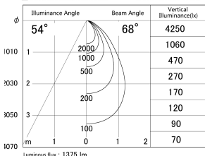
■ Direct Horizontal Illuminance DD139-1550WW9035
