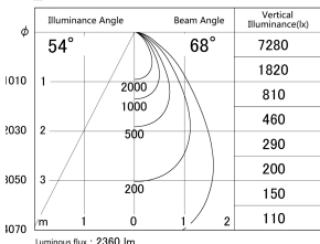
■ Direct Horizontal Illuminance DD139-2550WW9035
