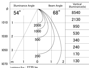
■ Direct Horizontal Illuminance DD139-3050WW9040
