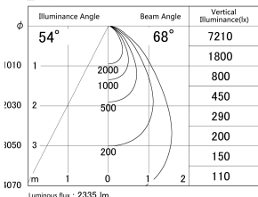
■ Direct Horizontal Illuminance DD139-2550WB9027
