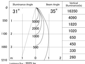
■ Direct Horizontal Illuminance DD139-2030WB9030
