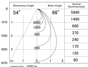
■ Direct Horizontal Illuminance DD139-2050WB9035
