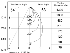
■ Direct Horizontal Illuminance DD139-1550WB9040
