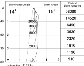
■ Direct Horizontal Illuminance DD139-2015WB9040
