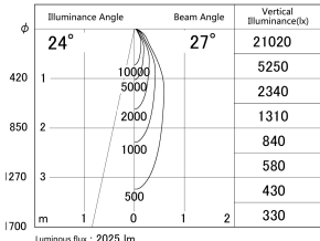
■ Direct Horizontal Illuminance DD139-2020WB9040
