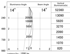
■ Direct Horizontal Illuminance DD139-1515MW9027D
