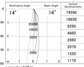
■ Direct Horizontal Illuminance DD139-2015MW9030D
