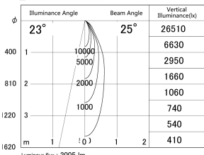
■ Direct Horizontal Illuminance DD139-2020MW9030D
