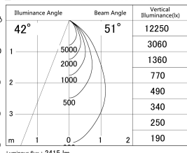
■ Direct Horizontal Illuminance DD139-2550MW9030D
