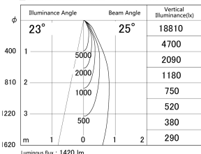
■ Direct Horizontal Illuminance DD139-1520MW9035D
