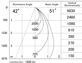
■ Direct Horizontal Illuminance DD139-2050MW9035D
