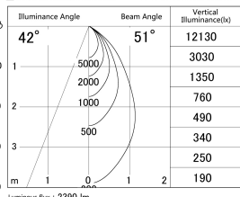
■ Direct Horizontal Illuminance DD139-2550MW9035D
