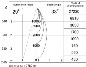
■ Direct Horizontal Illuminance DD139-3030MW9035D
