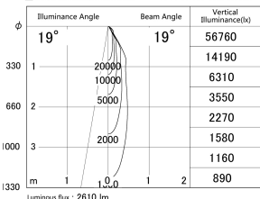
■ Direct Horizontal Illuminance DD139-2520MW9040D
