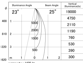
■ Direct Horizontal Illuminance DD139-1520MB9030D
