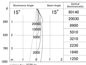
■ Direct Horizontal Illuminance DD139-3015MB9040D
