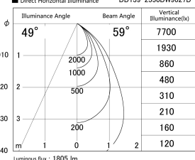
■ Direct Horizontal Illuminance DD139-2550DW9027D
