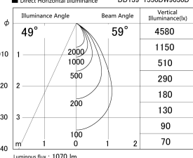
■ Direct Horizontal Illuminance DD139-1550DW9030D
