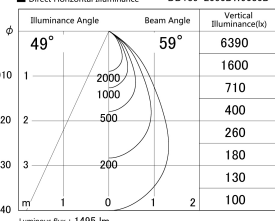
■ Direct Horizontal Illuminance DD139-2050DW9030D
