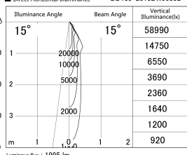
■ Direct Horizontal Illuminance DD139-2515DW9030D
