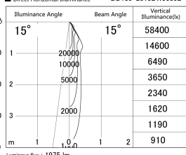
■ Direct Horizontal Illuminance DD139-2515DW9035D
