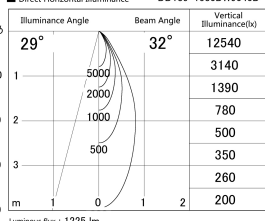
■ Direct Horizontal Illuminance DD139-1530DW9040D
