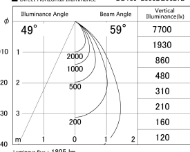
■ Direct Horizontal Illuminance DD139-2550DB9027D
